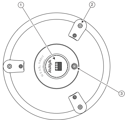
Rear Drawing
