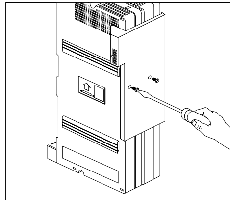
Figure 2-6. Fastening the 2-Slot Carrier
